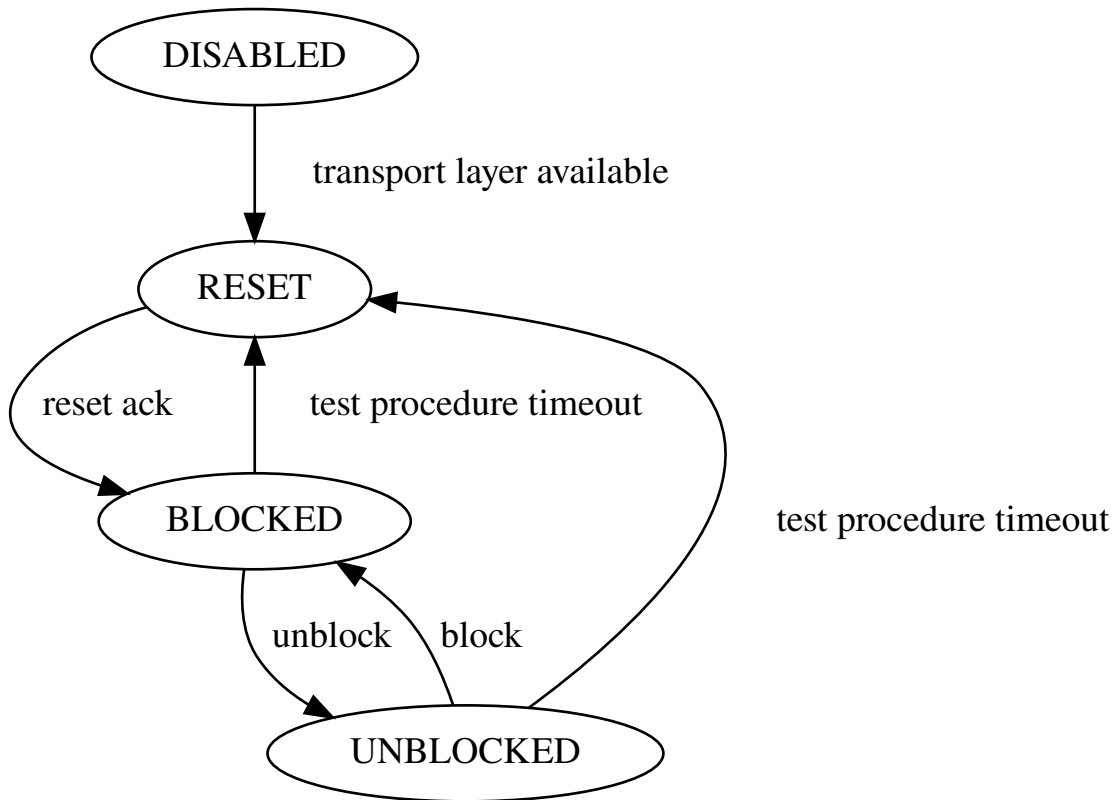
Figure 5: Simplified state diagram for RESET BLOCK UNBLOCK NSVCs
