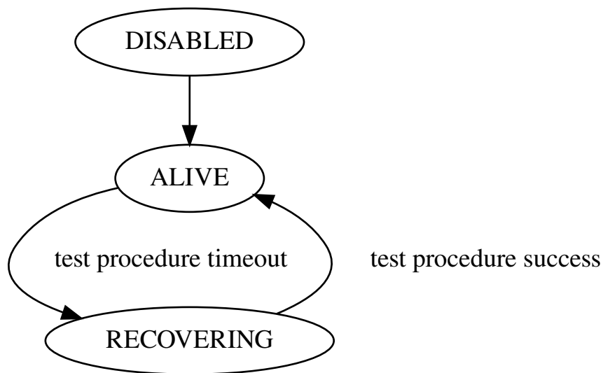
Figure 6: Simplified state diagram for IP-SNS/UDP
