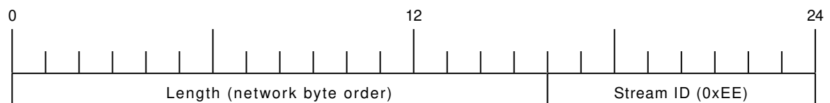
Figure 3: IPA header for control protocol
