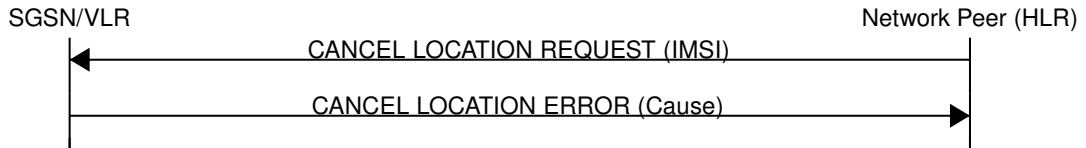
Figure 19: Cancel Location (Error Case)
