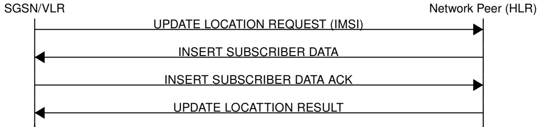
Figure 16: Update Location (Normal Case)
