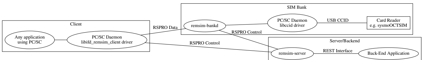
Figure 2: Overall osmo-remsim architecture using libifd_remsim_client
