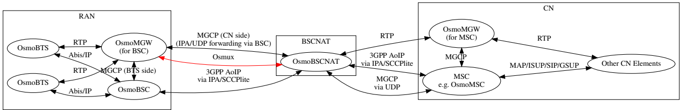
Figure 8: Sample node diagram of a 3GPP AoIP using A/IP with IPA/SCCP lite network and BSC-NAT with Osmux enabled
