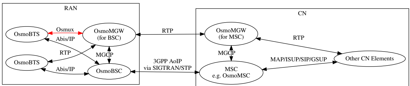
Figure 10: Sample node diagram of Osmux enabled in the Abis interface
