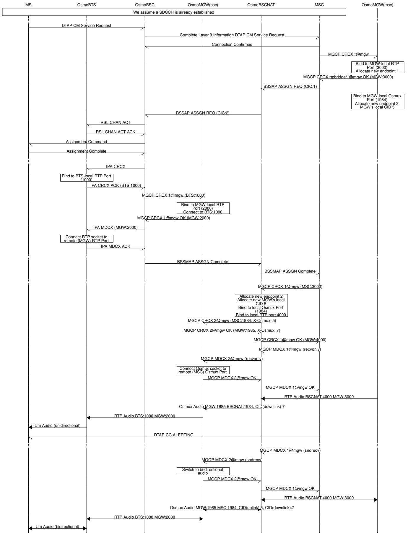
Figure 9: MO-call with Osmux enable on 3GPP AoIP using A/IP with IPA/SCCP lite with a BSC-NAT between BSC and MSC
