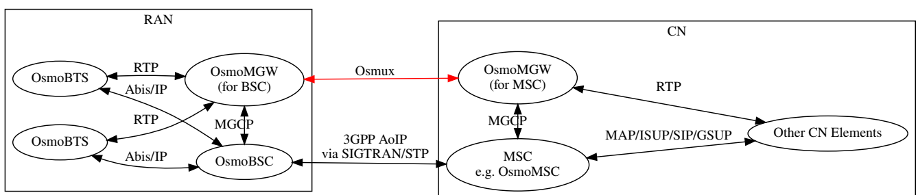
Figure 4: Sample node diagram of a 3GPP AoIP network with Osmux enabled
