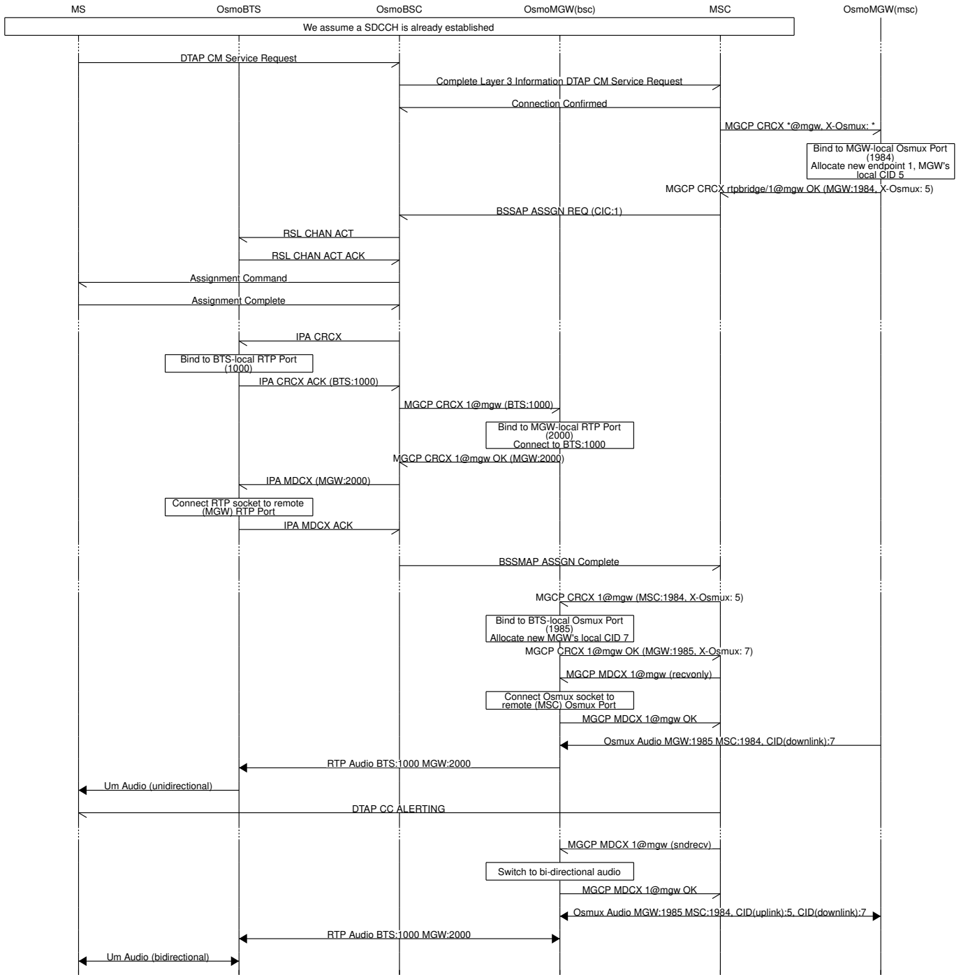
Figure 7: MO-call with Osmux enable on 3GPP AoIP using A/IP with IPA/SCCP-lite
