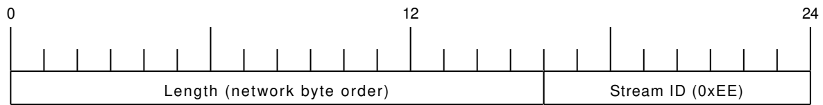
Figure 3: IPA header for control protocol
