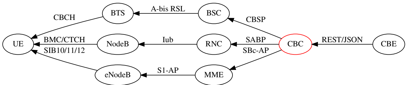
Figure 1: Role of the CBC inside the 3GPP network architecture
